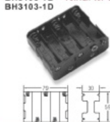
BH3103-1A BH3103-1B BH3103-1D FOR TEN "AA" CELLS
