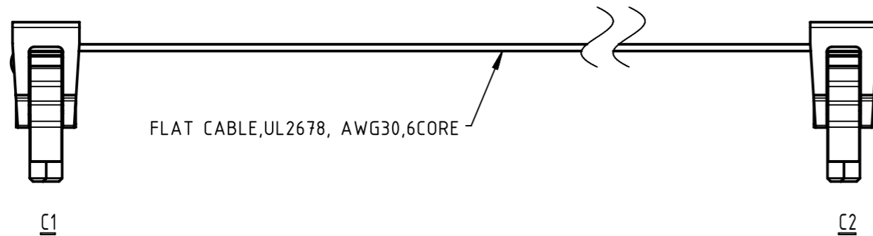
HAR-FLEX 6P FEMALE IDC CONNECTOR WITH SR
