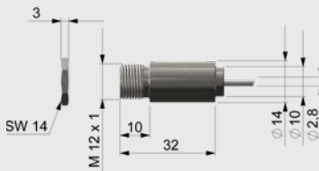
Sensing head (built-in CF lens)
