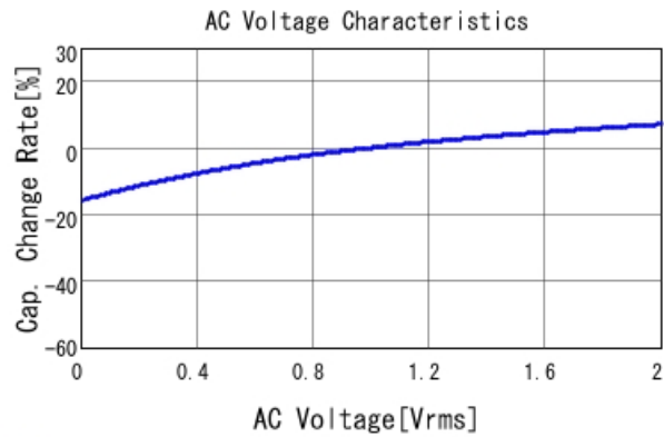
■ GCJ188R91E334KA01 C-AC Voltage capchange, DCOV, 25.0d
