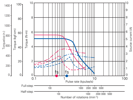
Source voltage : AC100V, Operating current : 4A/phase — Pull-Out torque [JL1=15.3x10 -4 kg-m 2 (83.65 oz-in 2 ) Use the rubber coupling] - - - Source current (TL=MAX), - - - Source current (TL=0)
