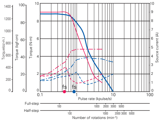
Source voltage : AC100V, Operating current : 4A/phase — Pull-Out torque [JL1=43x10 -4 kg-m 2 (235.10 oz-in 2 ) Use the rubber coupling] - - - Source current (TL=MAX), - - - Source current (TL=0)
