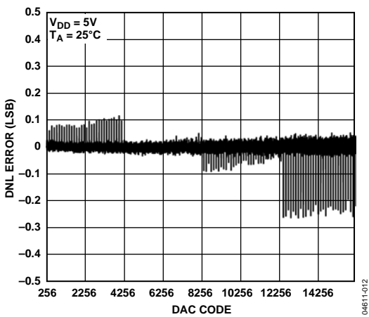
Figure 13. Typical DNL
