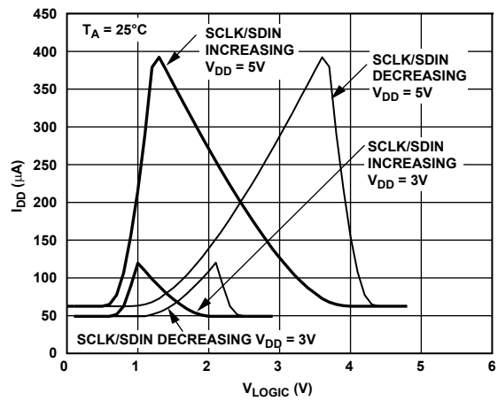
Figure 32. SCLK/SDIN vs. Logic Voltage
