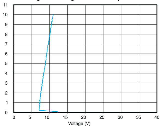
Figure 4. D+, D- Transmission Line Pulser Plot (100 ns Pulse, 10 ns Rise Time)
