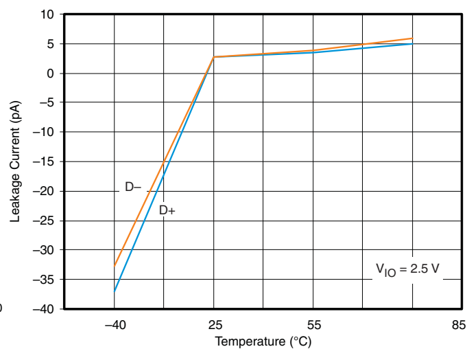
Figure 2. Leakage Current vs Temperature
