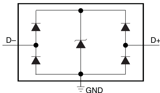
DBZ/DRT Circuit
