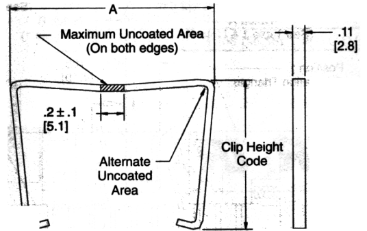
Short/Long Socket Retainer Clip
