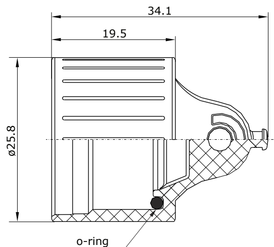
Main Dimensions protection cap
