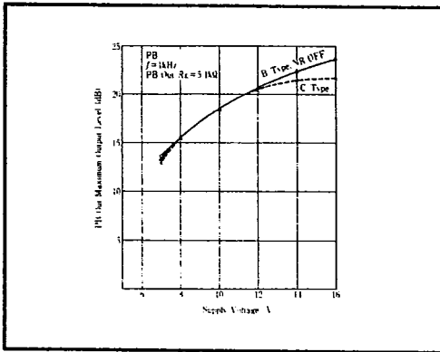
Figure 18 PB Out Maximum Output Level vs Supply Voltage
