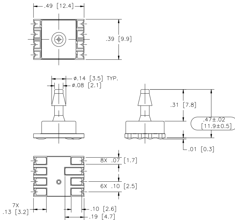
Model: MS4515-TPvoxxxyC
