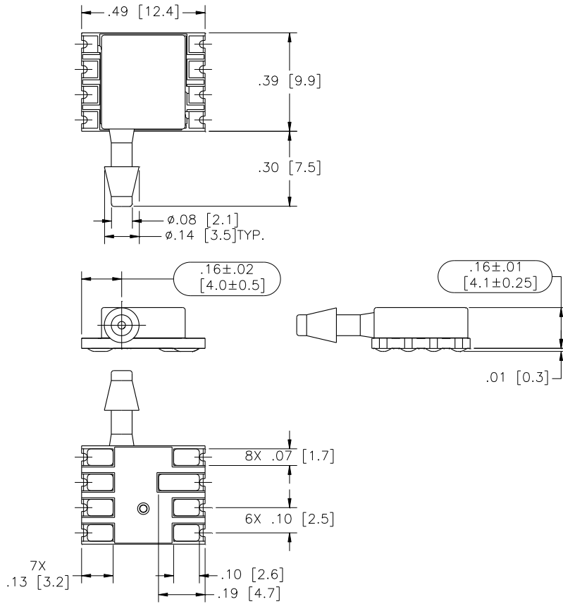
Model: MS4515-TPvoxxxyC
