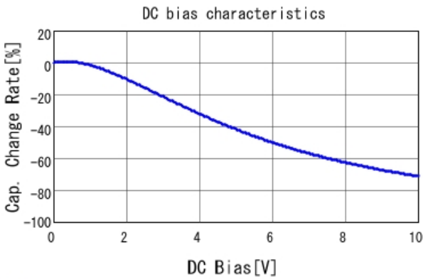
■ GRT32EC81A476KE13 C-DC bias capchange, 25.0degC, AC0.
