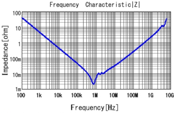
■ GRT32EC81A476KE13 |Z| DCOV, 25degC
