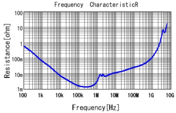
■ GRT32EC81A476KE13 R DCOV, 25degC
