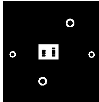
Figure 52. Evaluation Board Layout (Component Side)
