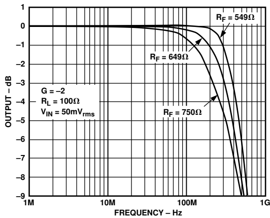
Figure 35. -3 dB Bandwidth vs. Frequency, G = -2
