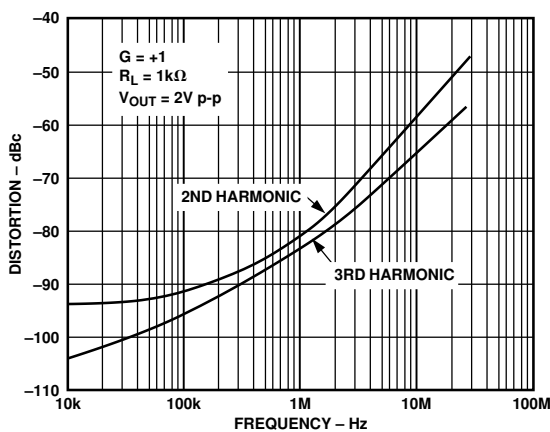
Figure 18. Distortion vs. Frequency, R_L = 1\ k\Omega
