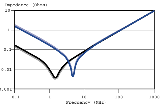
FIGURE 7. Impedance versus Frequency X5R Dielectric
