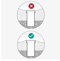
Make correct drainage (min. 300 mm.)
