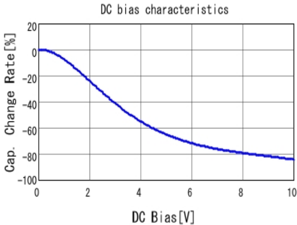
■ GRT155R61A475ME13 C-DC bias capchange, 25.0degC, AC1V
