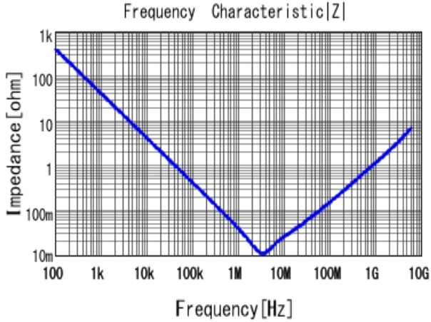
■ GRT155R61A475ME13 |Z| DCOV, 25degC
