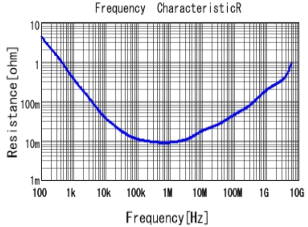
■ GRT155R61A475ME13 R DCOV, 25degC
