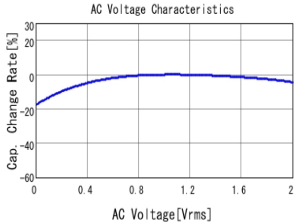
■ GRT155R61A475ME13 C-AC Voltage capchange, DCOV, 25.0d
