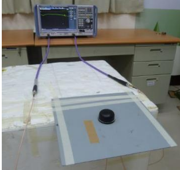
Figure 1. Impedance measurements.
