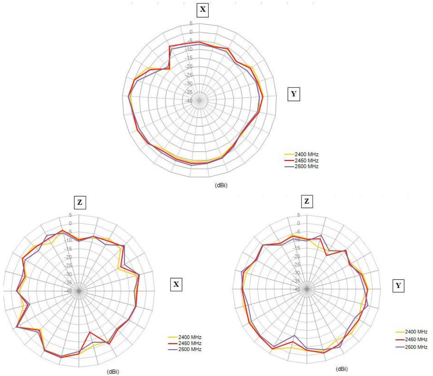
Figure 19. 2D Radiation Pattern at 2400MHz band
