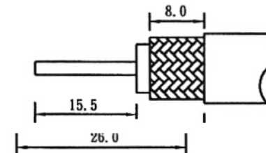
recommended Cable Stripping
