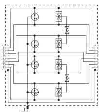
Basic circuit diagram DPA CLE IP66
