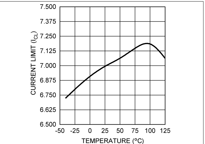
Figure 2. Current Limit vs Temperature
