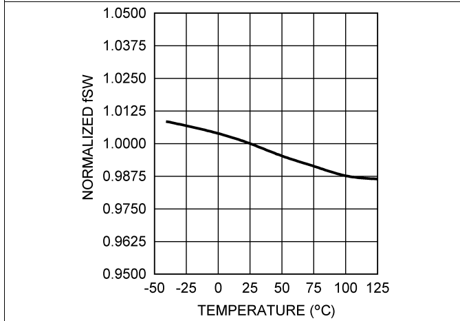
Figure 3. Normalized Switching Frequency vs Temperature
