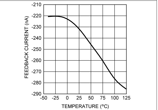
Figure 4. Feedback Bias Current vs Temperature
