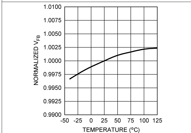
Figure 5. Normalized Feedback Voltage vs Temperature
