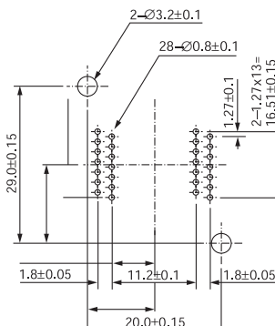
SOP IC51-0302-904 (30 Pins)
