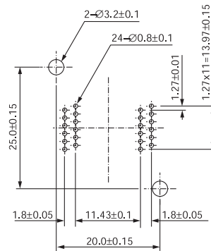
SOP IC51-0242-269-1 (24 Pins)
