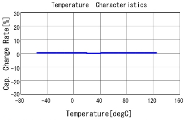
■ GCM1555C1H821FA16 C-Temp. capchange, DCOV, AC1Vrms
