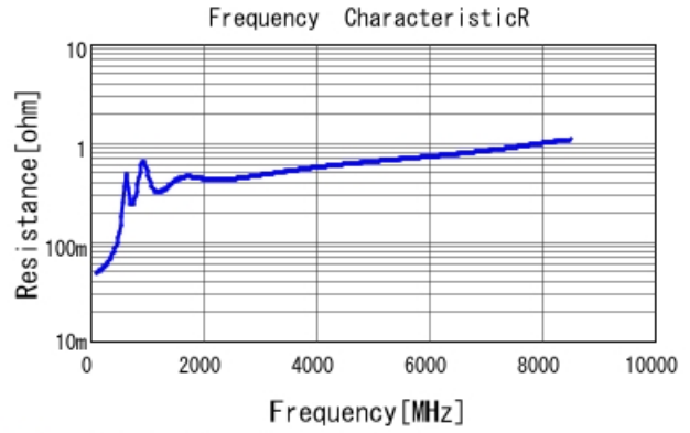
■ GCM1555C1H821FA16 R DCOV, 25degC
