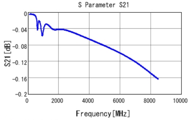
■ GCM1555C1H821FA16 S21 DCOV, 25degC
