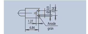
Bohrbild · Drilling Scheme
