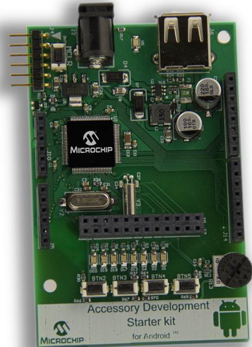
Microchip's PIC24F MCU Accessory Development Starter Kit for Android™ (Part # DM240415)
