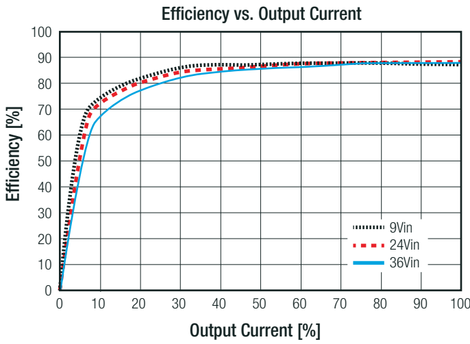
RPA20-2412SAW
