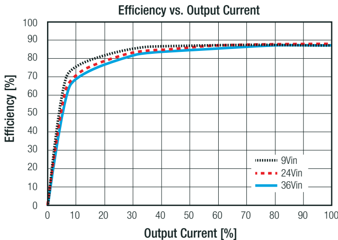
RPA20-2412DAW
