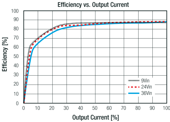
RPA20-2415SAW
