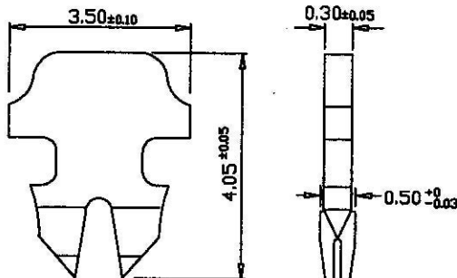
"2": 2 PRONGS FOR SOLID WIRE(SS) 單芯線用大拐角型金片
