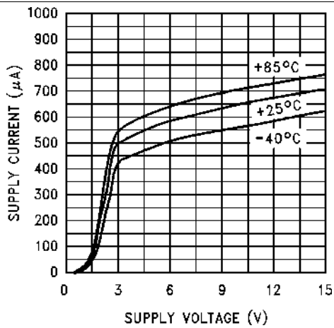
Figure 27. Supply Current vs Supply Voltage
