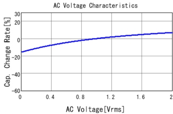
■ GCJ188R91E394KA01 C-AC Voltage capchange, DC0V, 25.0d
