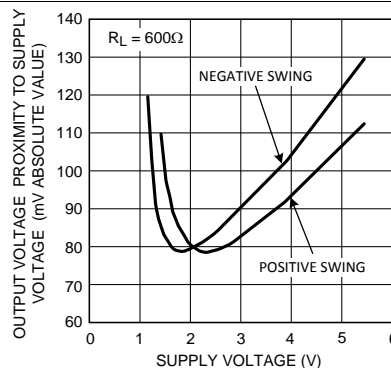
Figure 4. Output Voltage Swing vs. Supply Voltage
