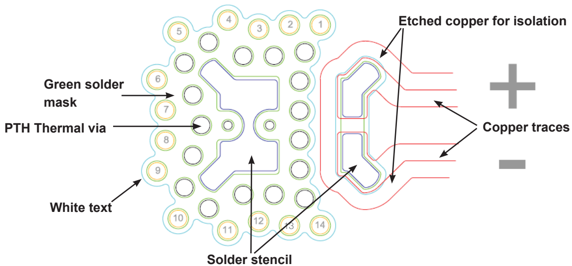
Figure 11. Outline of the recommended pad layout for a LUXEON LED (top view). See Figure 8 for more illustrations. There is 0.5mm spacing between the thermal and electrical pads.
