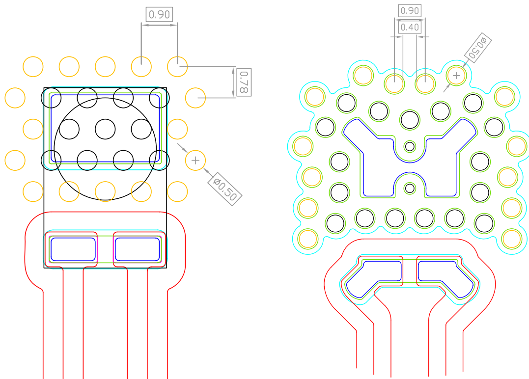
Figure 15. Recommended finished diameter and spacing dimensions for both open via PTH and filled and capped via design. All dimensions are in mm.
