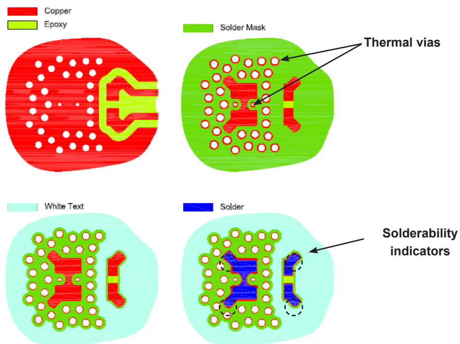
Figure 8. Recommended layout for a LUXEON LED with open via PTH board.
