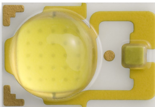
Figure 5. Typical metallization pattern of a LUXEON LED (configuration B). The TVS in this configuration resides in a separate pocket on the ceramic substrate.
