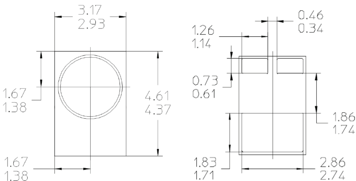
Figure 39. Mechanical dimensions of the LUXEON LED. All dimensions are in mm.
