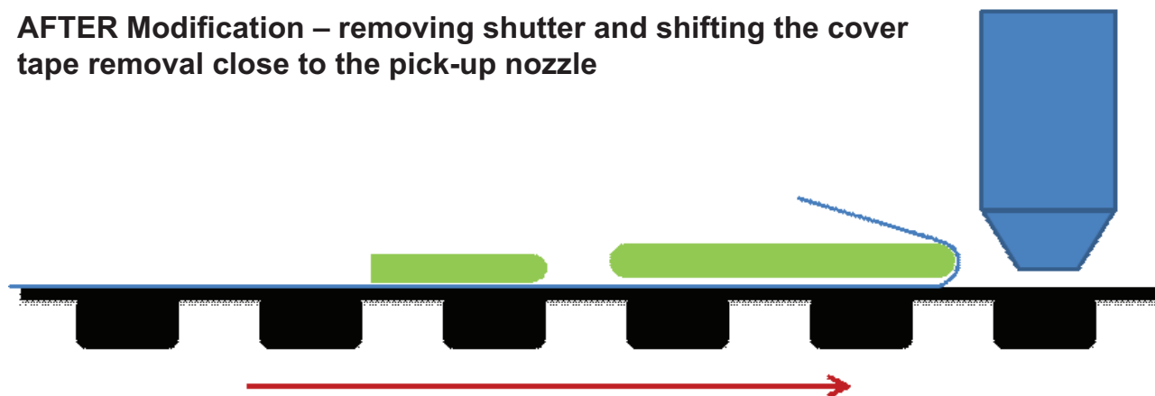
Figure 38. Minor modifications to the pick and place machine minimize the chance of damage to the silicone lens of the LUXEON LED.
