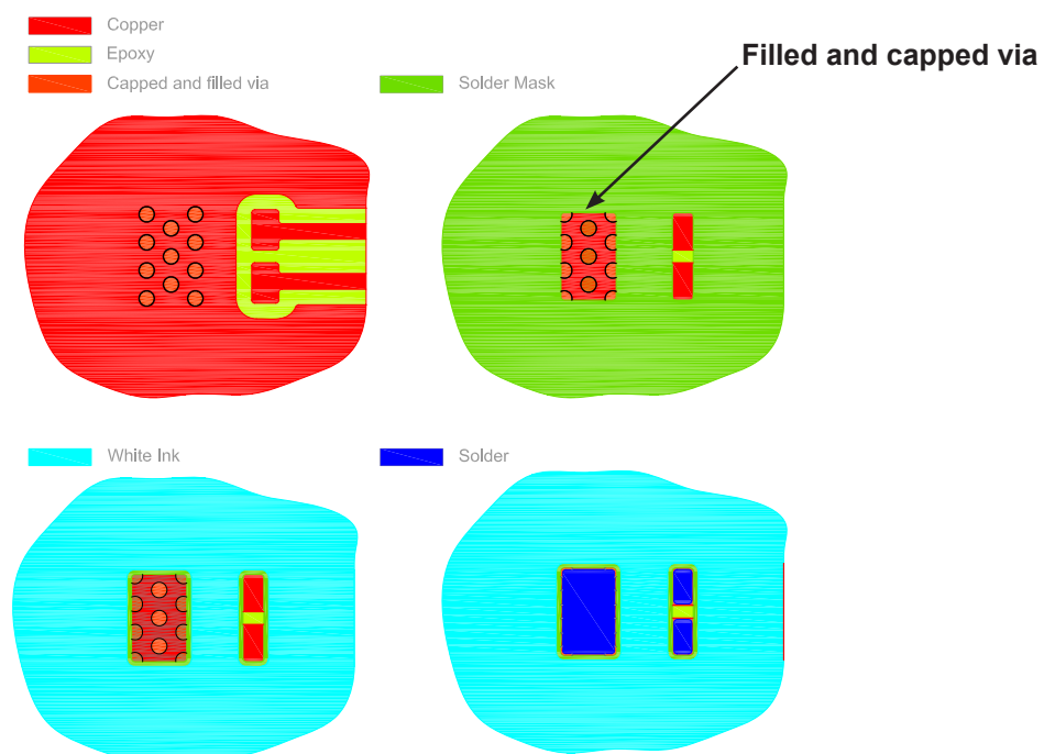
Figure 9. Recommended layout for a LUXEON LED with filled and capped vias.
