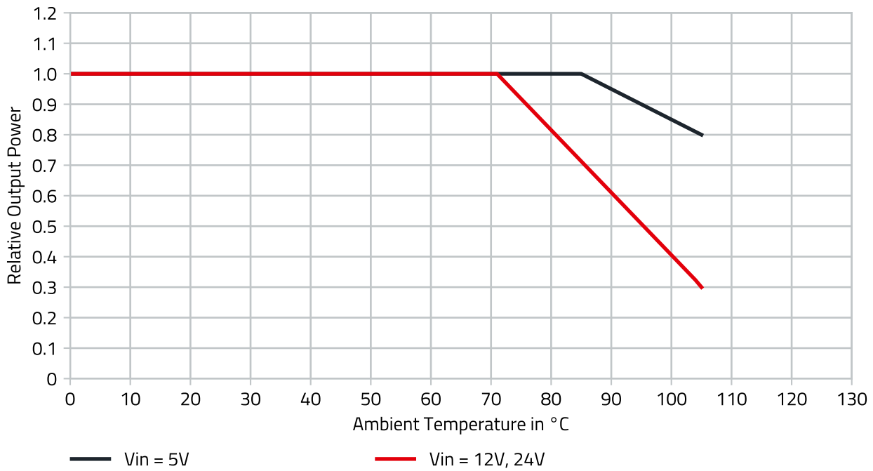
Figure 10: 1769405x41 output power thermal derating, V_{IN} = \text{Nom.} , I_{OUT} = 0.4A .
