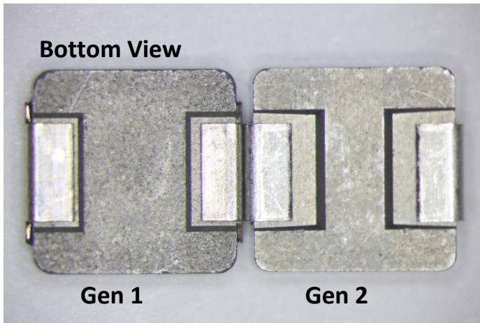
Figure 2. Shows an optical view of the bottom of the units.
