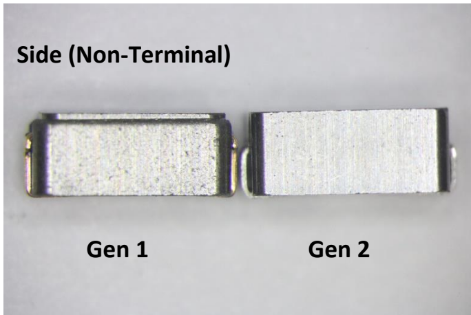
Figure 3. Shows an optical view of the Non-Leadframe side of the units.
