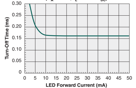
Typical Turn-Off Time vs. LED Forward Current ( T_A=25^\circ C , I_L=120mA_{DC} )
