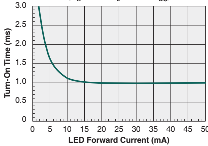
Typical Turn-On Time vs. LED Forward Current ( T_A=25^\circ C , I_L=120mA_{DC} )
