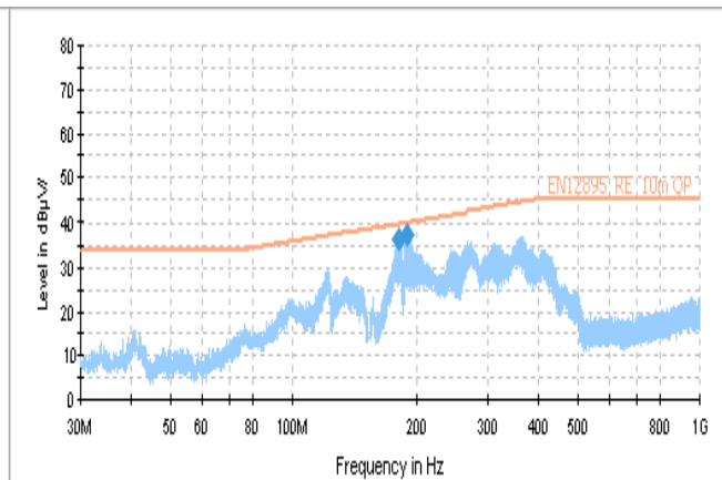
Figure 16: test result(Horizontal)
