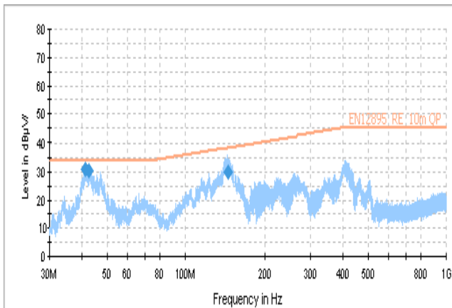
Figure 15: test result(Vertical)
