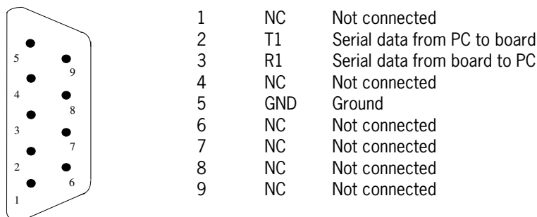
Figure 9. The pin configuration of J10 (9 pole SUB-D female).
