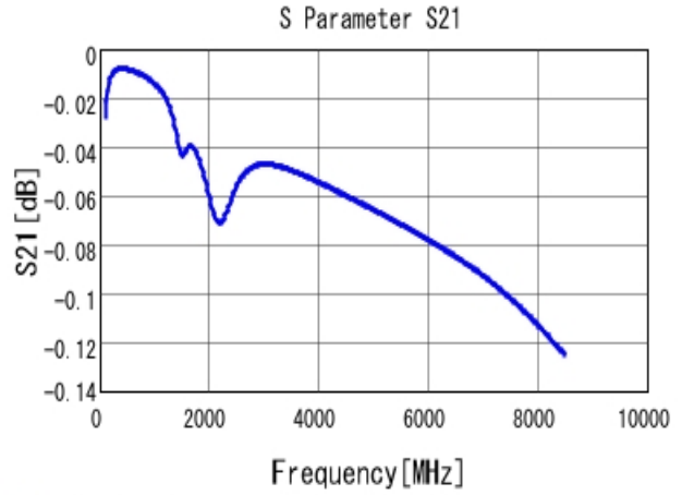
■ GRM0335C1E221JA01 S21 DCOV, 25degC
