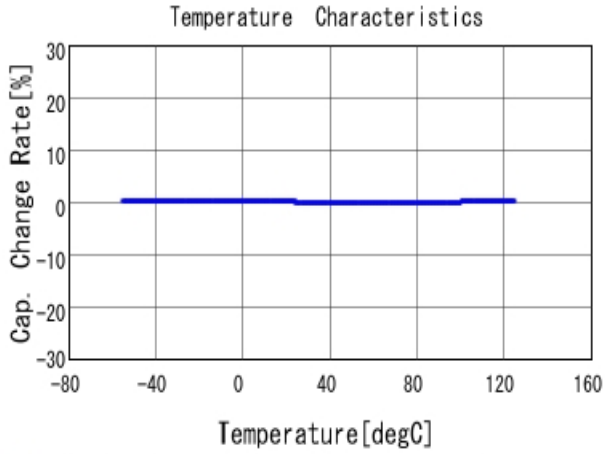
■ GRM0335C1E221JA01 C-Temp. capchange, DCOV, AC1Vrms
