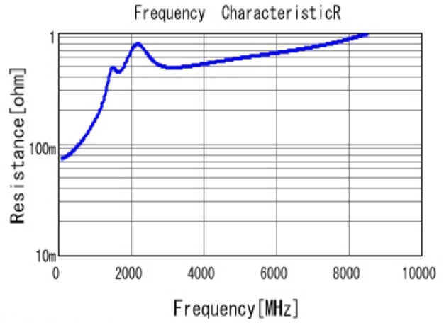
■ GRM0335C1E221JA01 R DC0V, 25degC
