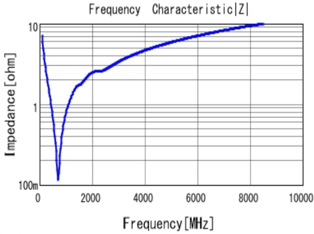
■ GRM0335C1E221JA01 |Z| DC0V, 25degC
