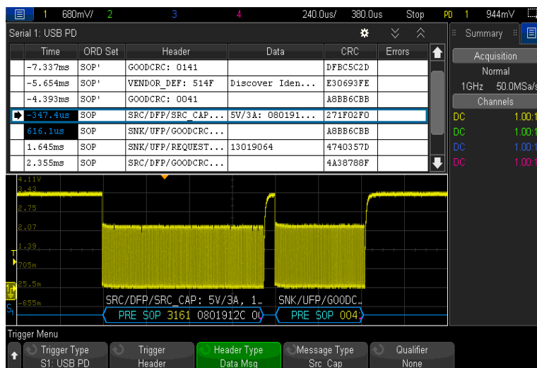
Figure 14. USB PD decode on an InfiniiVision X-Series
