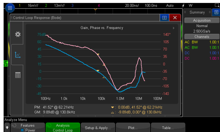
Figure 10. Control loop response gain & phase measurement.
