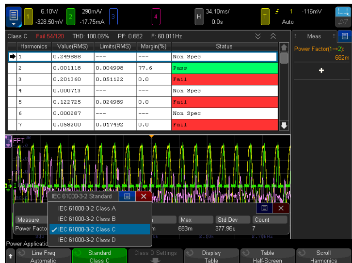
Figure 2. Current harmonics measurement based on IEC 61000-3-2 standards.
