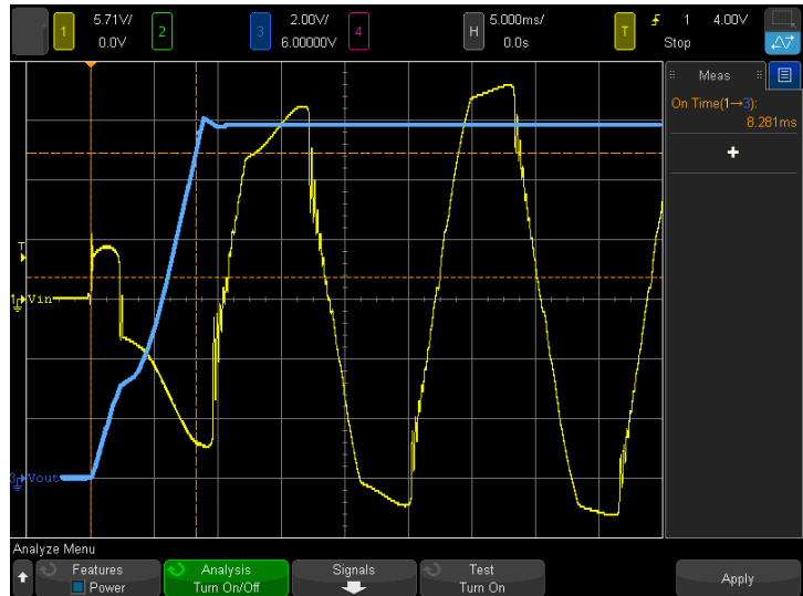
Figure 7. AC-to-DC turn-on time measurement.
