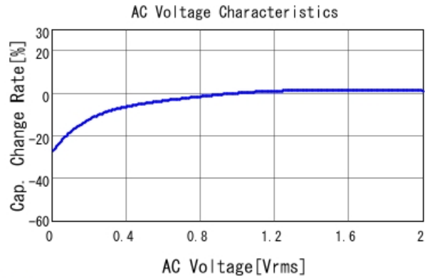
■ GRM188Z71A106KA73 C-AC Voltage capchange, DCOV, 25.0d
