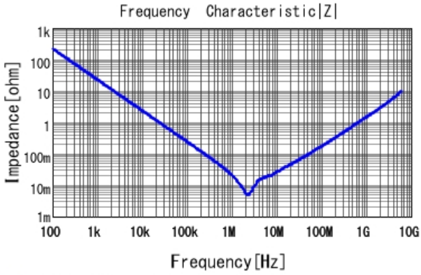
■ GRM188Z71A106KA73 |Z| DCOV, 25degC
