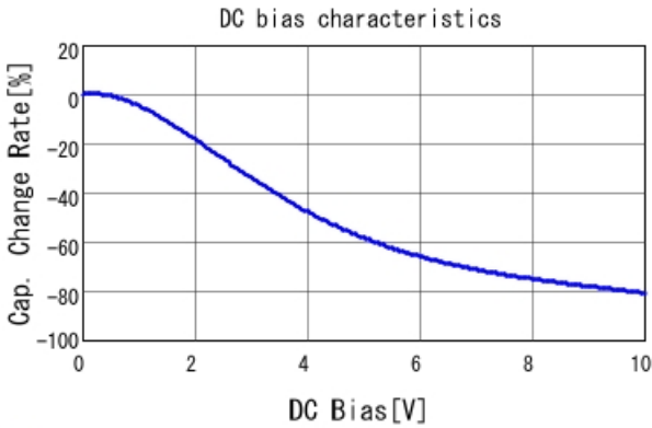
■ GRM188Z71A106KA73 C-DC bias capchange, 25.0degC, AC1V
