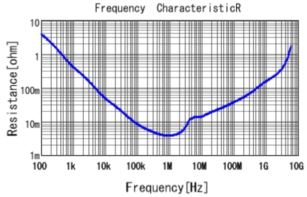
■ GRM188Z71A106KA73 R DCOV, 25degC
