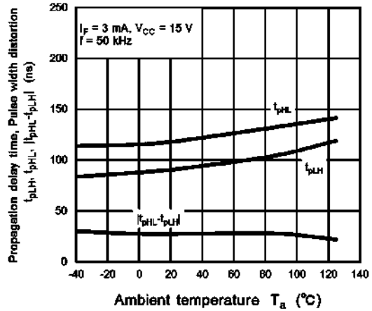
Fig. 12.2.16 t_{pHL}, t_{pLH}, |t_{pHL} - t_{pLH}| - T_a (Test Circuit Fig. 12.1.7)
