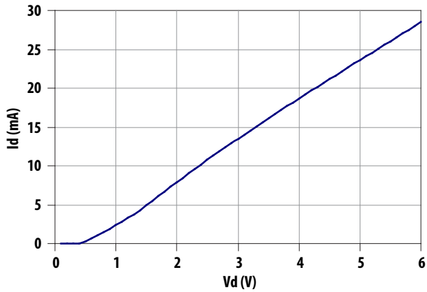
Figure 7. Total Current [1]
