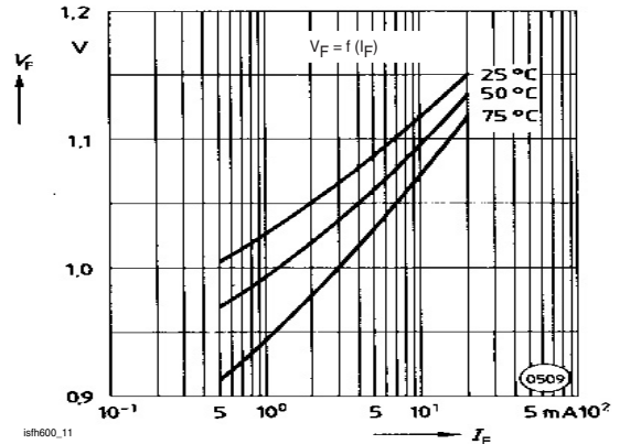
Figure 11. Forward Voltage
