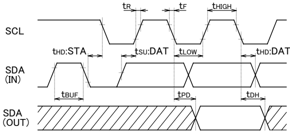
Figure 1-(a). Serial Input / Output Timing
