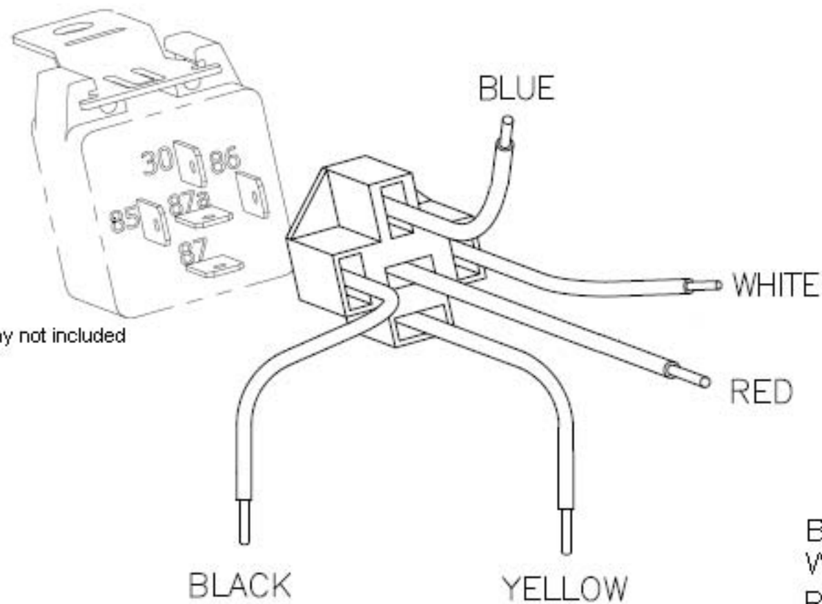
Part #26-1942 Five Pin Relay Socket
