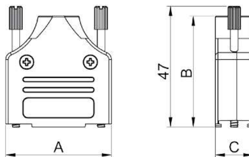
D-Sub-Hood
