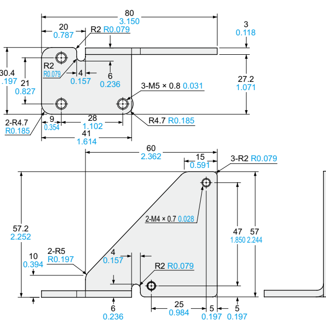
MS-LX-2 Sensor mounting bracket (Optional)
