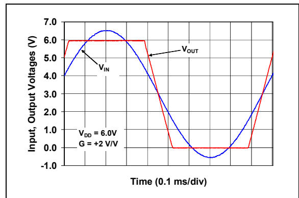
FIGURE 2-30: The MCP6401/1R/1U Shows No Phase Reversal.
