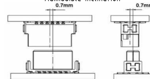
Admissible inclination
