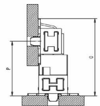
straight male
