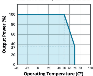
TEMPERATURE DERATING CURVE (full load 400W with 25 CFM) VOF-450C-12-CFS, VOF-450C-15-CFS
