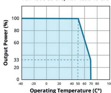
TEMPERATURE DERATING CURVE (full load 450W with 25 CFM) VOF-450C-24-CFS, VOF-450C-27-CFS VOF-450C-36-CFS, VOF-450C-48-CFS
