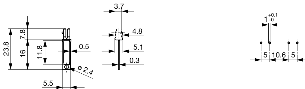
Drilling diagram
