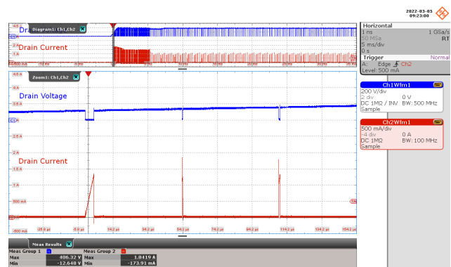
Figure 33 – Drain Voltage and Current Waveforms. 265 VAC, 80 mA Output. Drain Voltage: 200 V / div., 5 ms / div. Drain Current: 500 mA / div., 5 ms / div. Zoom = 20 \mu s / div. I_{DS(MAX)} = 1.84 A, V_{DS(MAX)} = 406.32 V.
